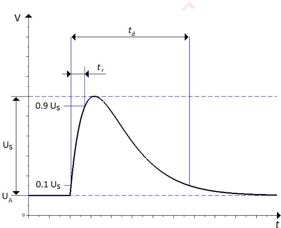
Figure 2.1: The surge voltage U_S is the pulse maximum voltage disregarding the offset voltage U_A . The rise t_r time is defined as the time elapsed from 0.1 to 0.9 times the surge voltage on the rising edge of the pulse. The duration t_d is defined as the time from 0.1 times the maximum voltage on the rising edge, back to the same level of the falling edge.
