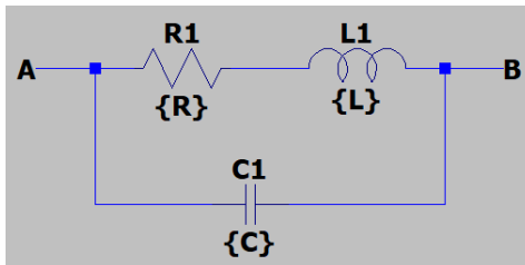
Figure 2.3: At high frequencies a resistors parasitic inductance and capacitance will affect the behavior of the circuit.
