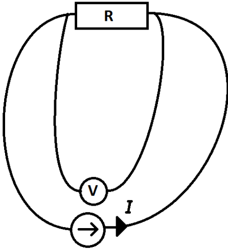
Figure 2.4: When measuring a low value resistor, the Kelvin connection can be used to determine the resistance at the point where the voltmeter is connected without the resistance in the probe leads affecting the result.
