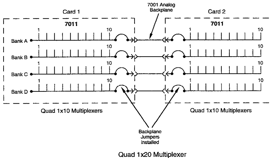
Figure 2-12 Multiplexer input expansion example
