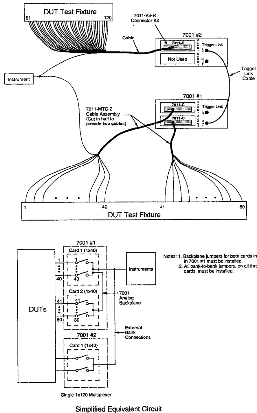
Figure 3-16 Two-mainframe system example (multi-pin connector card)
