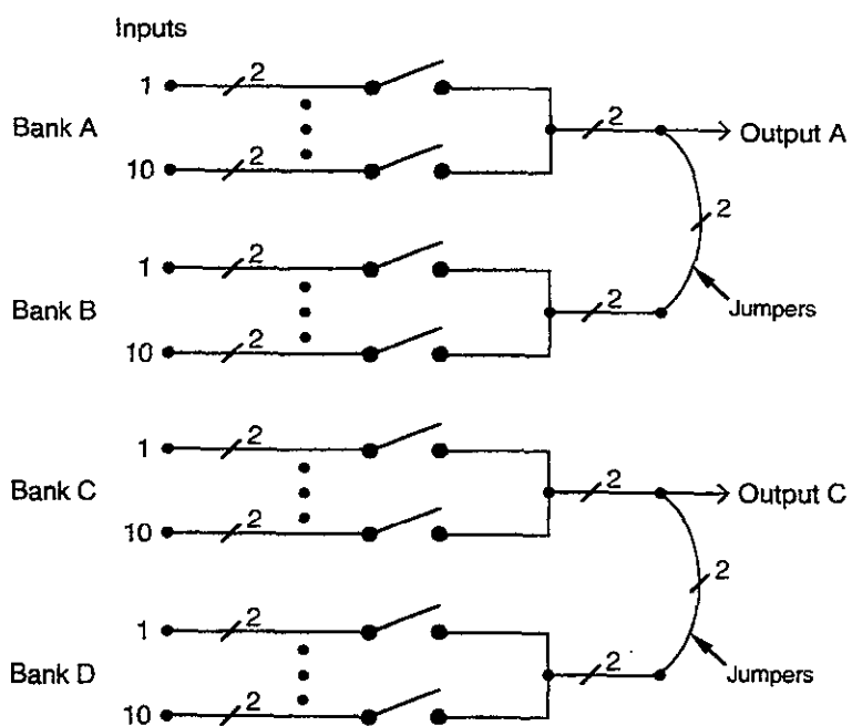
Figure 2-3 Two 1 x 20 multiplexer configuration (jumpers installed)
