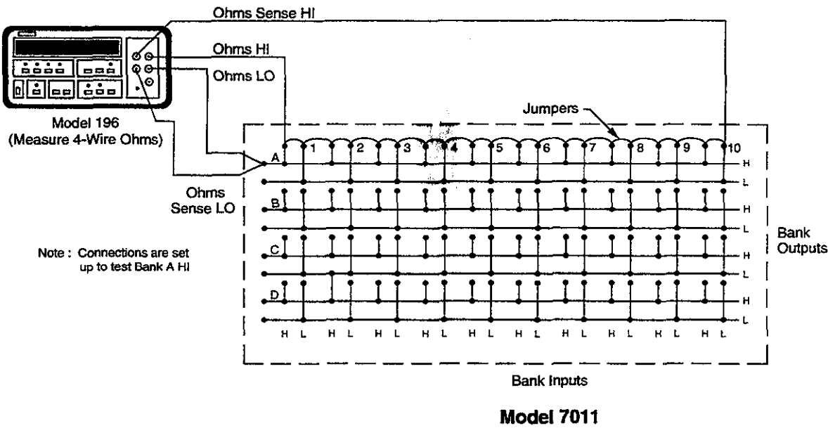
Figure 5-1 Path resistance test connections
