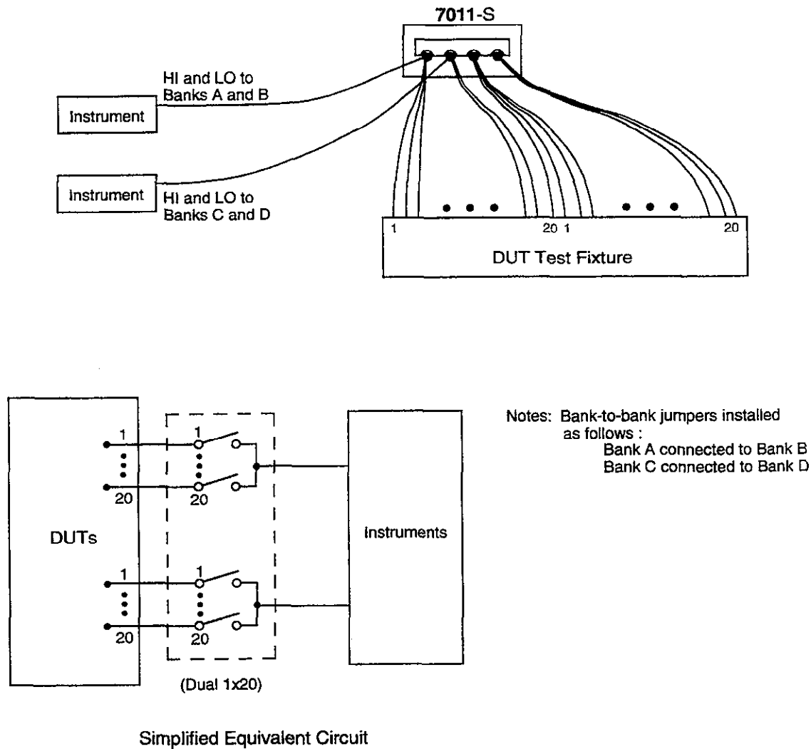
Figure 3-13 Single card system example (screw terminal connector card)
