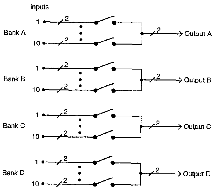
Figure 2-2 Four 1 x 10 multiplexer configuration (jumpers not installed)
