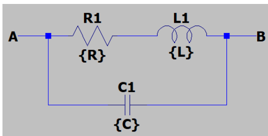
Figure 2.6: At high frequencies a resistors parasitic inductance and capacitance will affect the behavior of the circuit.
