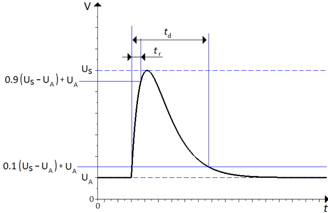
Figure 2.5: Illustration of load dump Test A. Note the difference of U_S compared to all the other pulses. To minimize the risk of misunderstandings, only the way of specifying U_S as the other pulses do will be used unless otherwise stated.
