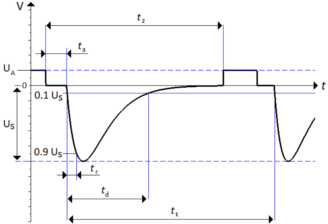
Figure 2.2: Illustration of test pulse 1.
