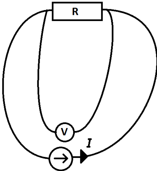
Figure 2.7: When measuring a low value resistor, the Kelvin connection can be used to determine the resistance at the point where the voltmeter is connected without the resistance in the probe leads affecting the result.
