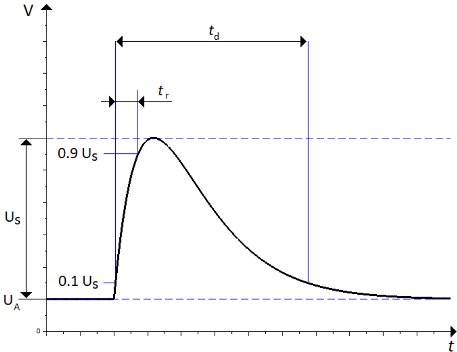
Figure 2.1: The surge voltage U_S is the pulse maximum voltage disregarding the offset voltage U_A . The rise t_r time is defined as the time elapsed from 0.1 to 0.9 times the surge voltage on the rising edge of the pulse. The duration t_d is defined as the time from 0.1 times the maximum voltage on the rising edge, back to the same level of the falling edge.
