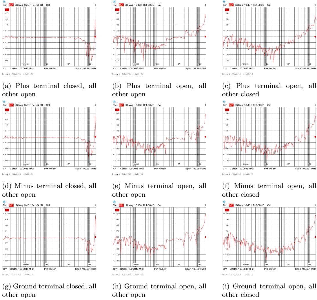
Figure 4.1: The S21 measurements for the attenuators
