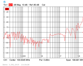
(h) Ground terminal open, all other open
