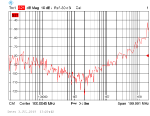
(c) Plus terminal open, all other closed
