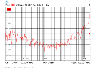
(i) Ground terminal open, all other closed
