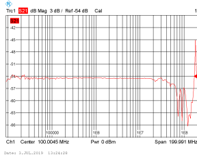
(a) Plus terminal closed, all other open
