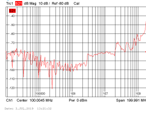
(b) Plus terminal open, all other open
