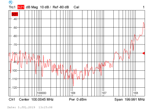
(f) Minus terminal open, all other closed
