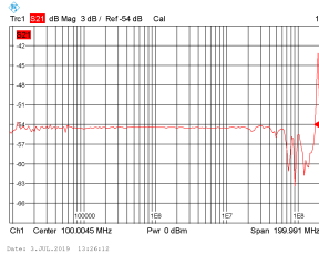
(g) Ground terminal closed, all other open
