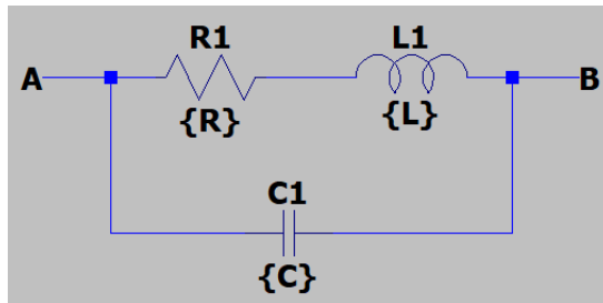
Figure 2.6: At high frequencies a resistors parasitic inductance and capacitance will affect the behavior of the circuit.
