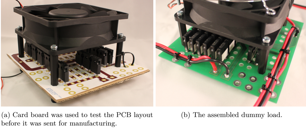
Figure 4.3: The resulting board was predicted using a card board mockup PCB.
