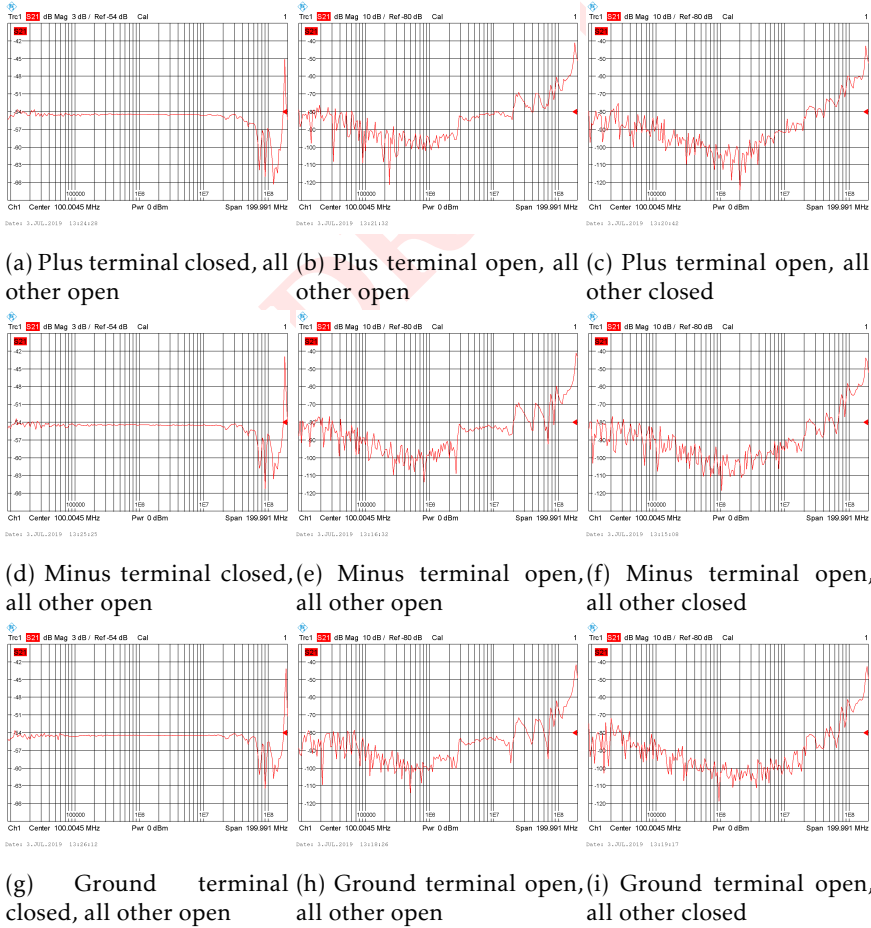
Figure 4.1: The measurements made on the attenuators
