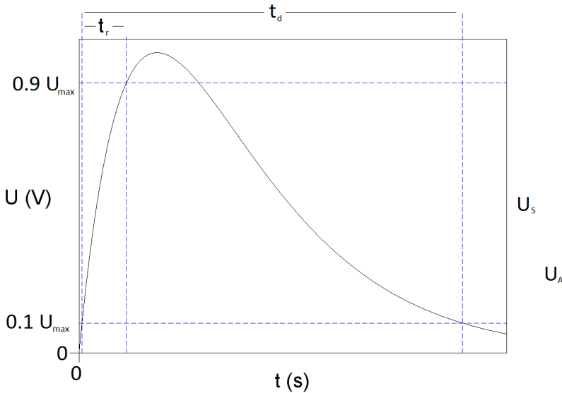
Figure 2.1: The rise time is defined as the time elapsed from 0.1 to 0.9 times the maximum voltage on the rising edge of the function. The duration is defined as the time from 0.1 times the maximum voltage on the rising edge, back to the same level of the falling edge.
