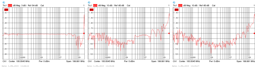
(g) Ground terminal closed, all other open (h) Ground terminal open, all other open (i) Ground terminal open, all other closed
