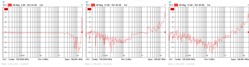
(a) Plus terminal closed, all other open (b) Plus terminal open, all other open (c) Plus terminal open, all other closed
