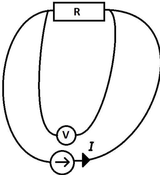
Figure 2.3: When measuring a low value resistor, the Kelvin connection can be used to determine the resistance at the point where the voltmeter is connected without the resistance in the probe leads affecting the result.
