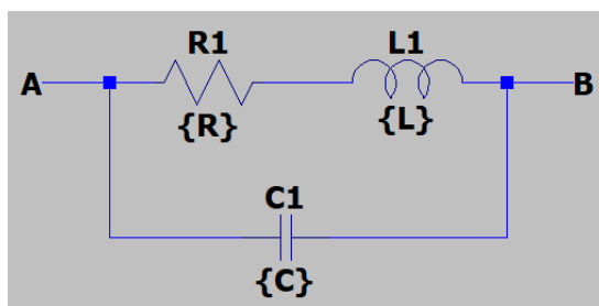
Figure 2.2: At high frequencies a resistors parasitic inductance and capacitance will affect the behavior of the circuit.
