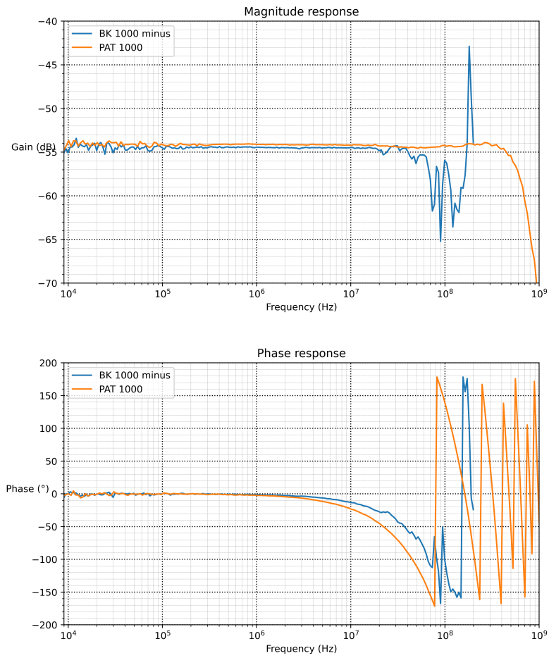
Figure 4.16: The constructed 1000\ \Omega attenuator compared to the commercial PAT 1000.
