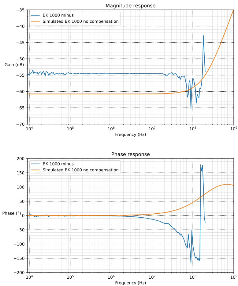
Figure 4.15: The simulated 1000\Omega attenuator compared to the constructed.
