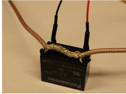
Figure 3.10: The relay measured with coaxial wires.
