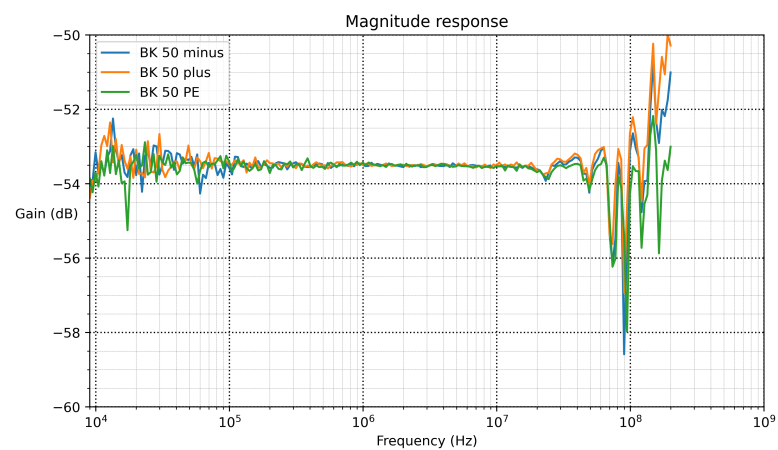
Figure 4.13: Comparison of the three different signal paths of the constructed 50\ \Omega attenuator.
