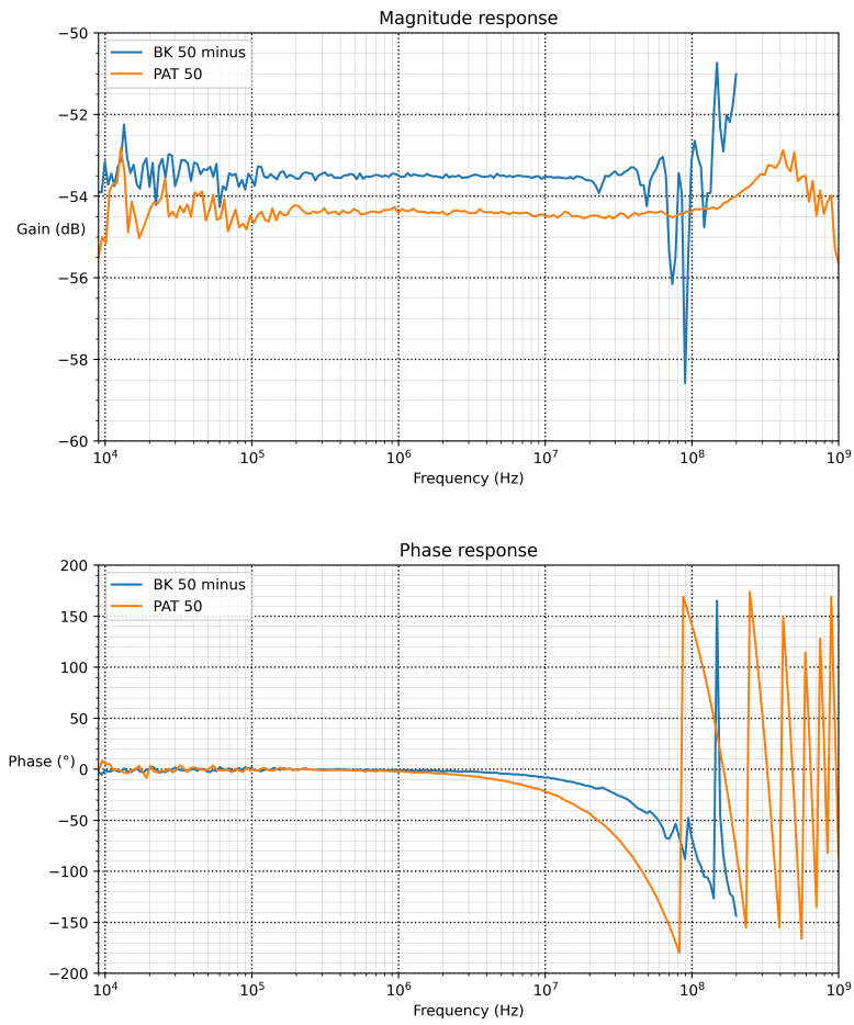
Figure 4.12: The constructed 50\ \Omega attenuator compared to the commercial PAT 50.
