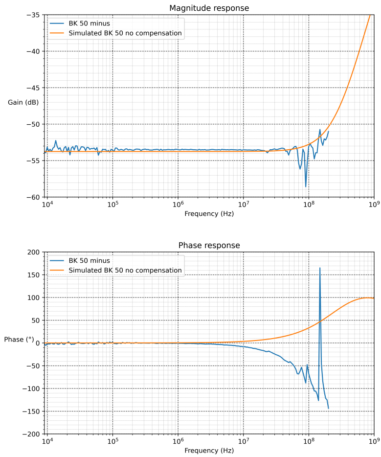
Figure 4.11: The simulated 50\Omega attenuator compared to the constructed.
