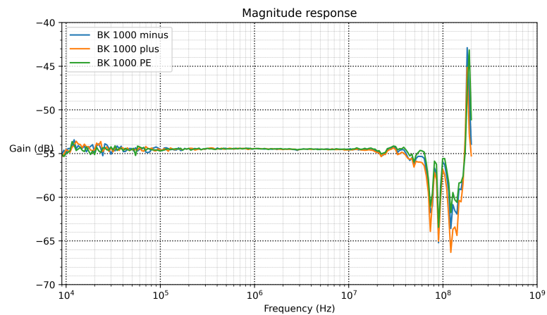
Figure 4.17: Comparison of the three different signal paths of the constructed 50\ \Omega attenuator.
