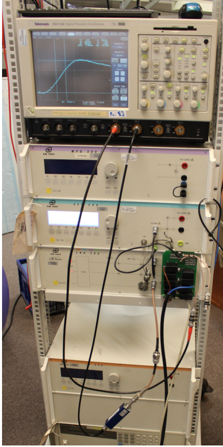
Figure 3.11: The time measurement setup. Both the commercial and the constructed attenuators were measured in this setup.
